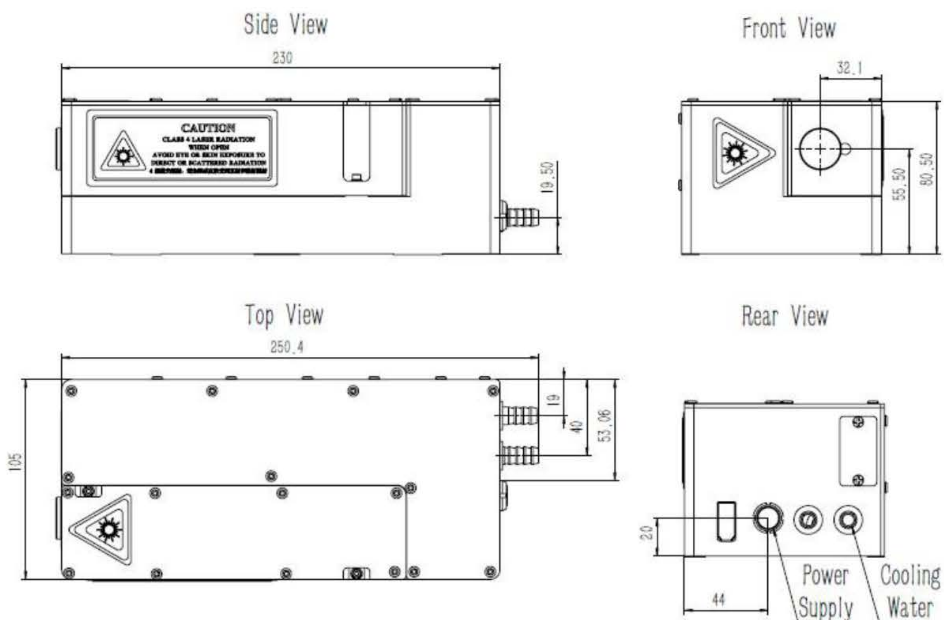
TINY-100L 355nm Laser Head Mechanical Specifications
